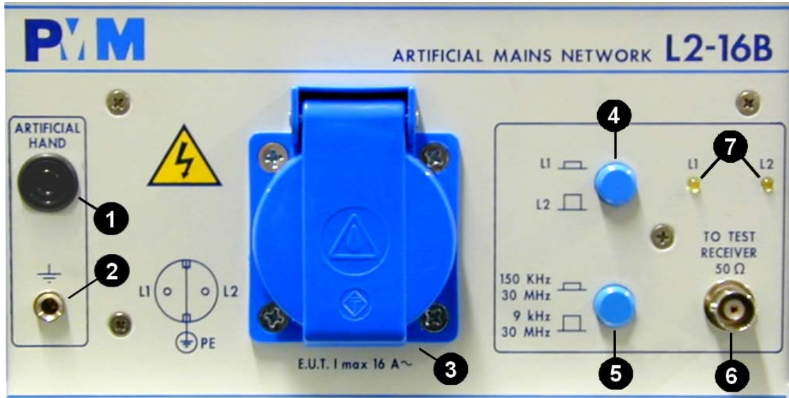
Fig. 3-5 Front Panel
